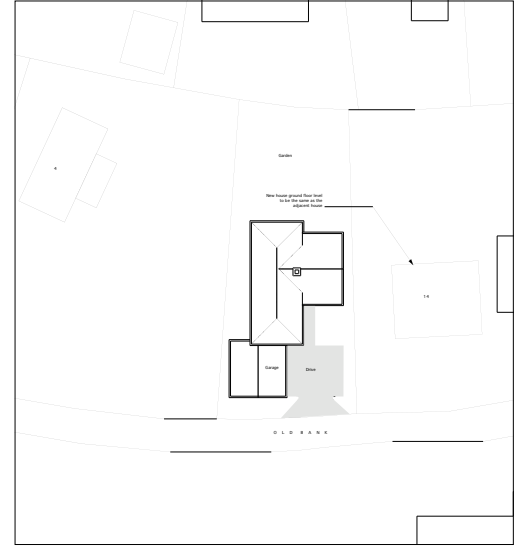
BLOCK PLAN 1:200
